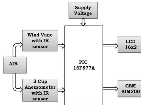
Figure 7 Block Diagram
